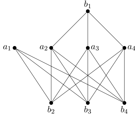
Figure 8: K(4, 4, 1) -subgraph.
